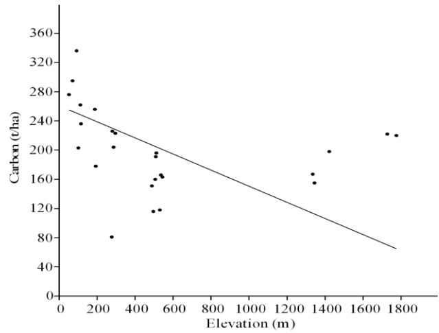
Fig. 4. Association between carbon (tC/ha) and elevation (m) of trees with dbh \geq 10 cm recorded in 25 1-ha plots in the Rumpi Hills Forest Reserve, Cameroon. The relationship has a correlation coefficient of 0.061, which is significantly different from a slope of zero ( p < 0.05 , y = -0.11x + 260.9 ).
