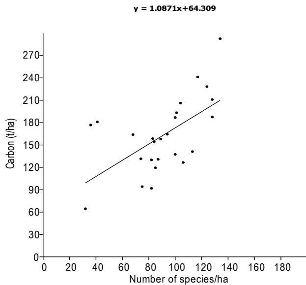
Fig. 5. Association between carbon (tC/ha) and number of species/ha with dbh \geq 10 cm recorded in 25 1-ha plots in the Rumpi Hills Forest Reserve, Cameroon; r^2 = 0.34 ; y = 1.0871x + 64.30 .
