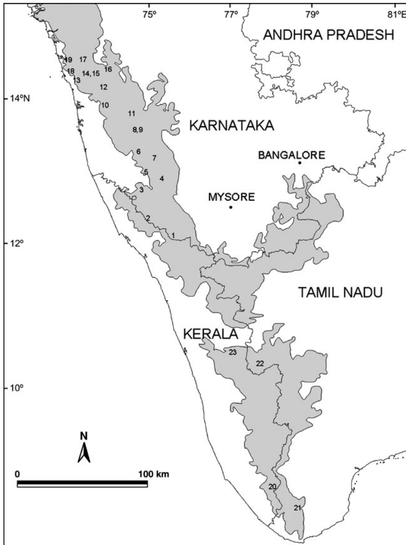
FIG. 1 South-western India, with the Western Ghats mountains (shaded areas) showing the locations of the known lion-tailed macaque populations in the states of Karnataka, Kerala and Tamil Nadu. The names of these numbered sites are given in Tables 2 and 4.
