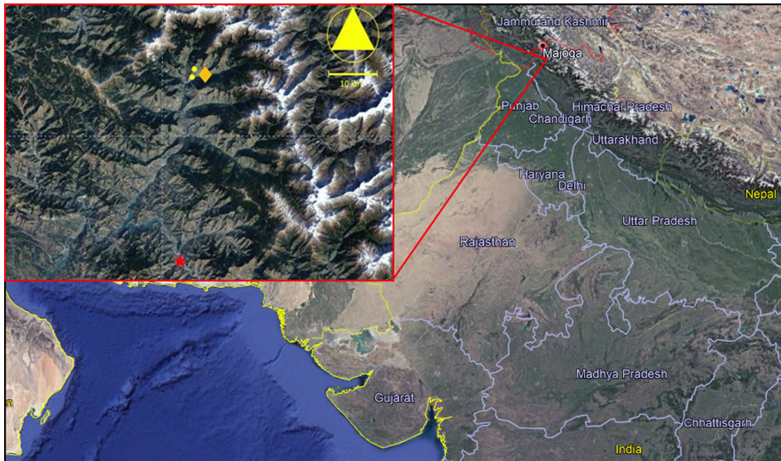
Figure 2. Naja oxiana Indian distribution (Yellow dots = N. oxiana observation locations, red star = Chamba, orange diamond = Majoga,)
